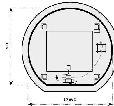
LED ROUND 60
