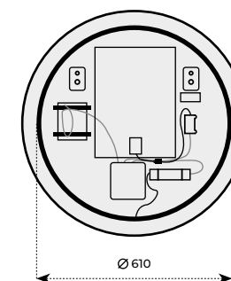
LED ROUND 80
