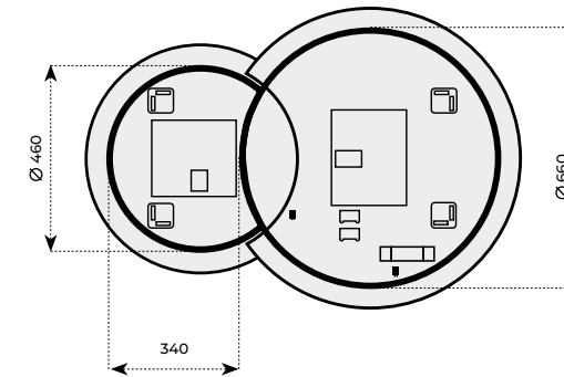
LED TWIN 80/60
