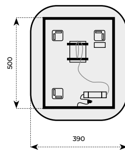
LED SHARON 60
